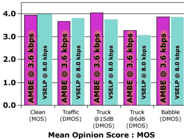
Figure 2. Inmarsat Voice Quality Test
