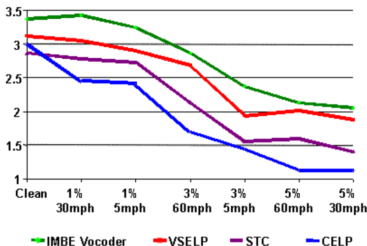
Figure 1. APCO Voice Quality Test
